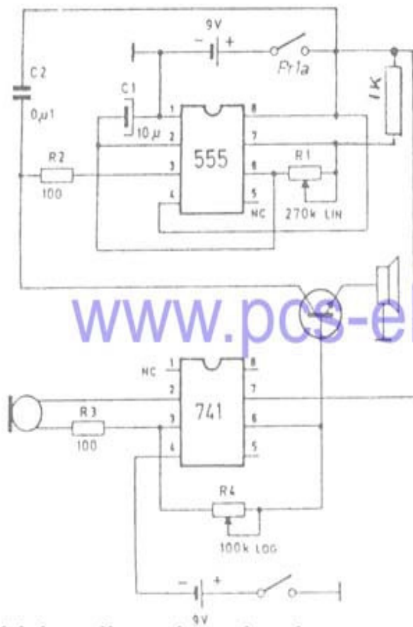
Voice distortion circuit
